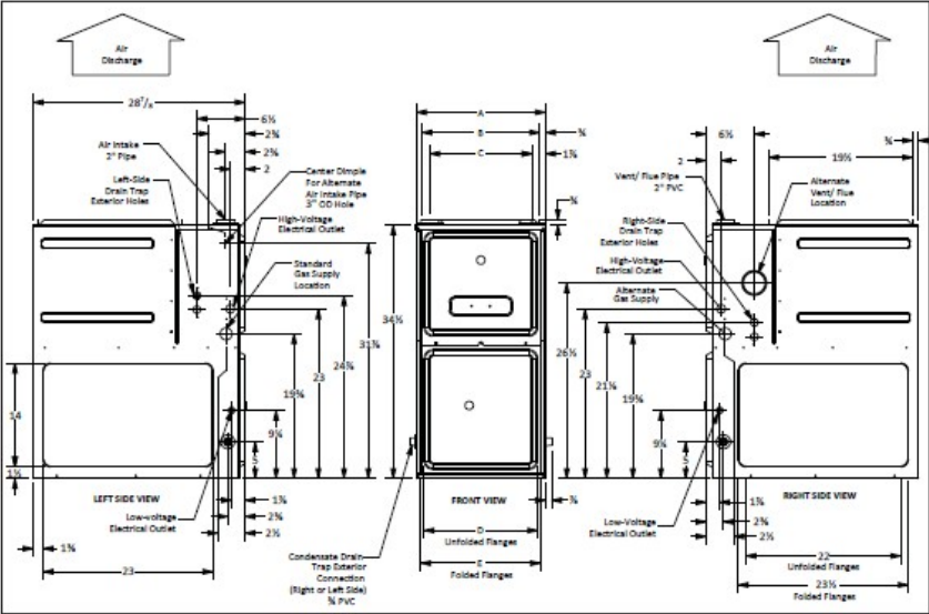
DR92SN DIMENSIONS
